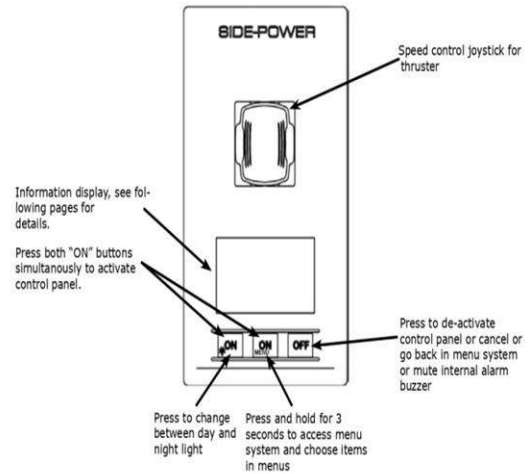
Panel Layout, PJC-211
